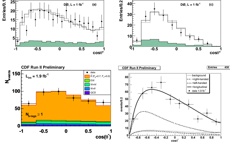
Figure 2: Reconstructed \cos\theta^* in the DZero \ell +jets channel (top left) and in the DZero dilepton channel (top right). Reconstructed \cos\theta^* in the CDF \ell +jets channel with the unfolding method (bottom left) and CDF template method (bottom right).
