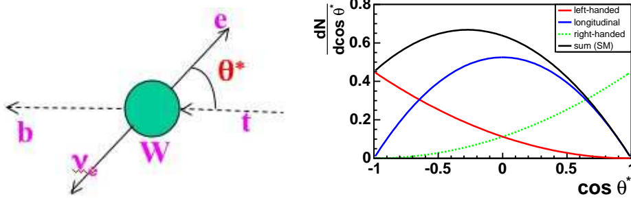
Figure 1: At left, the definition of the helicity angle \theta^* in the decay t \rightarrow bW \rightarrow bl\nu . At right, the distributions of \cos\theta^* for pure left-handed, pure right-handed, pure longitudinal samples, and the SM.
